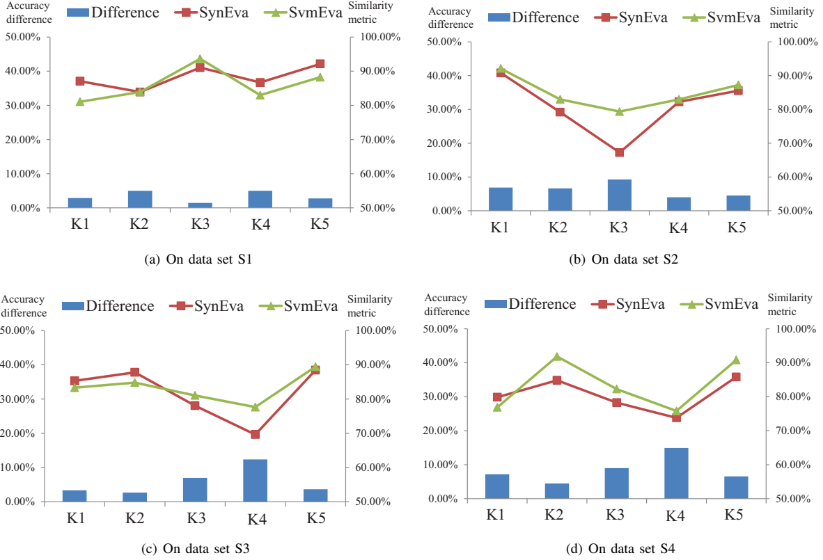
Fig. 4. Comparison of SynEva’s program synthesis techniques (whole structure + logic detail vs. whole logic)
