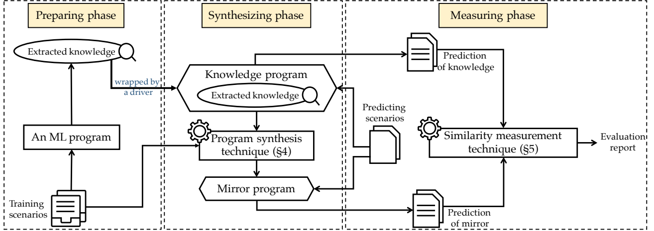
Fig. 1. SynEva overview.
