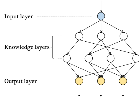
Fig. 2. Knowledge structure.
